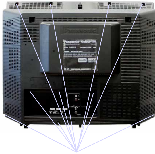
SCREWS Fig.2.
